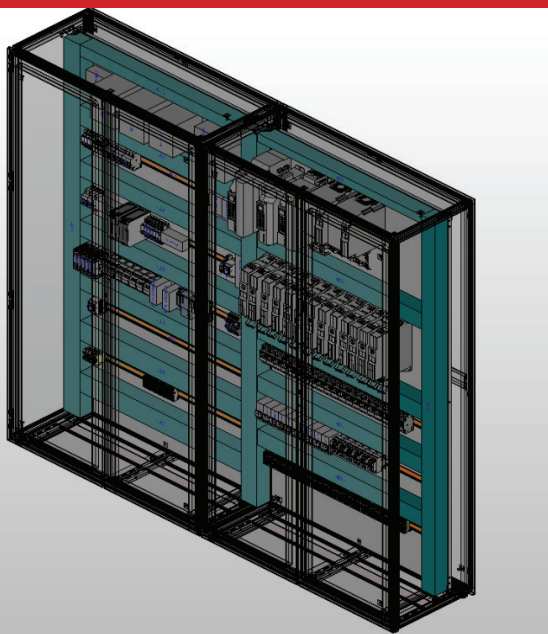
PICTURED: Layout and wiring design
